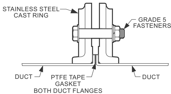
Floating Cast Ring
