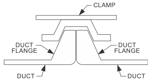
CROSS SECTION OF 2" (50.8) & 3" (76.2) PSP-EZ™ JOINT
