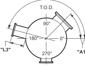
"D1" TAP ANGLE VIEW SPECIFY TAP ANGLE FROM 0° AT D1 END
