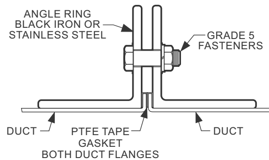
Floating Angle Ring
