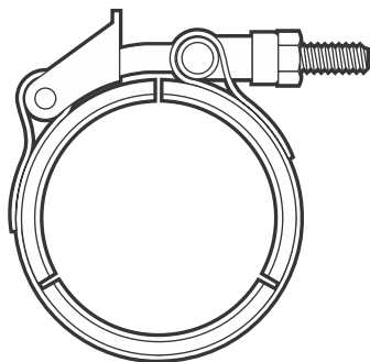
2" (50.8) & 3" (76.2) PSP-EZ™ CLAMP
