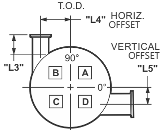
"D1" TAP OFFSET VIEW
