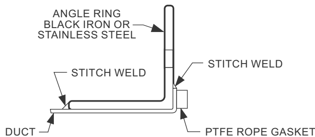
Stitch Welded Angle Ring
