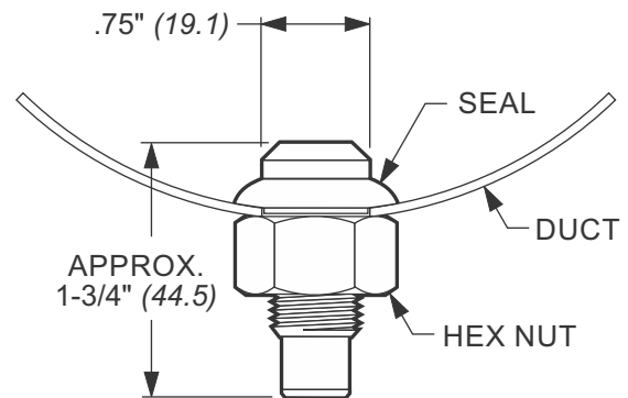
3/8" (9.5) TEST PORT
