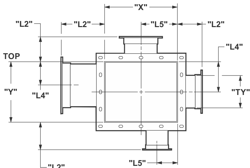
END VIEW
