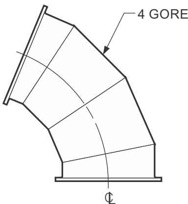
60° ELBOW
