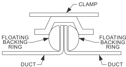
CROSS SECTION OF 4" (101.6) - 14" (355.6) PSP-EZ™ JOINT
