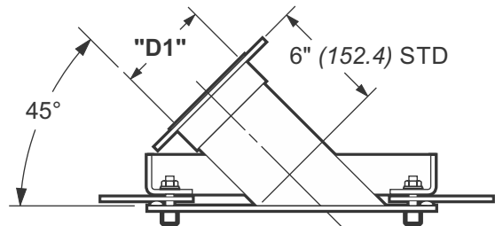
SECTION THROUGH DUCT - LATERAL TAP
