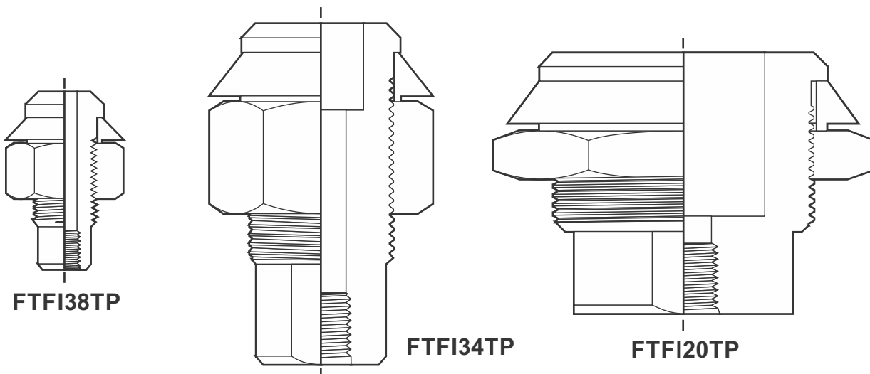
3/8" (9.5) TEST PORT
