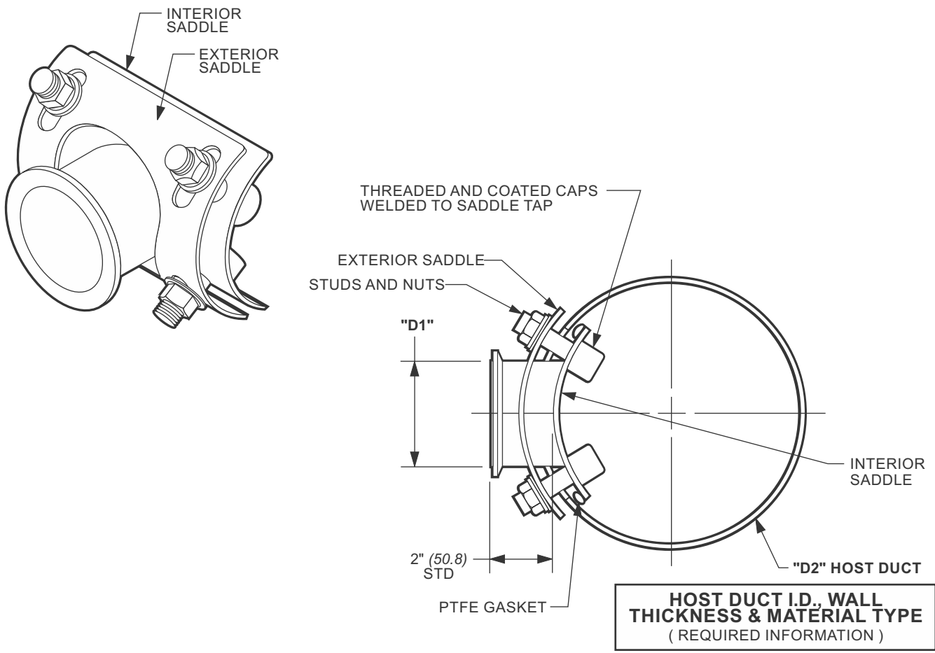
SECTION THROUGH DUCT
