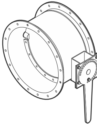
16" (406.4) - 48" (1219.2) DIA HIGH VALUE HEAVY DUTY INDUSTRIAL DAMPER (HVD)
