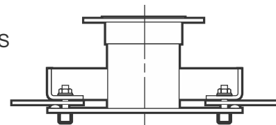
SECTION THROUGH DUCT - STRAIGHT TAP
