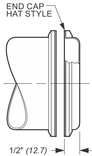
4" (101.6) - 14" (355.6) PSP-EZ™ CONFIGURATION
