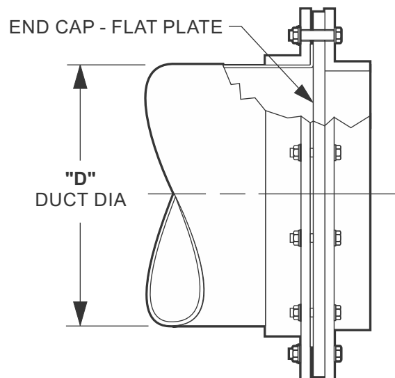
16" (406.4) - 120" (3048.0) ANGLE RING CONFIGURATION WITH ADDED SUPPORT ANGLE RING
